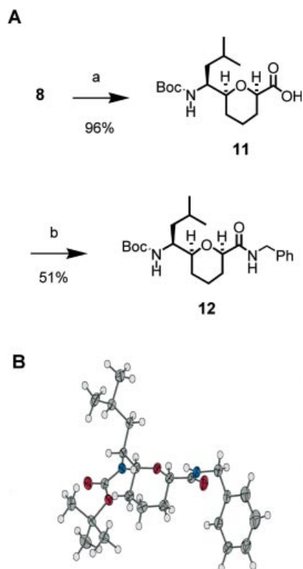
Scheme 3. A. Synthesis of THP-amino acid derivatives: a) i: (\text{COCl})_2 , DMSO, \text{Et}_3\text{N} , \text{CH}_2\text{Cl}_2 , -60 \rightarrow 0\text{ }^\circ\text{C} ; ii: \text{NaClO}_2 , \text{NaH}_2\text{PO}_4 , amylene, t\text{BuOH}/\text{H}_2\text{O} , 20\text{ }^\circ\text{C} ; b) benzylamine; HBTU, HOBT, DIEA, DMF/ \text{CH}_2\text{Cl}_2 , 20\text{ }^\circ\text{C} . B: solid state conformation of 12 obtained by X-ray crystal-structural analysis.
