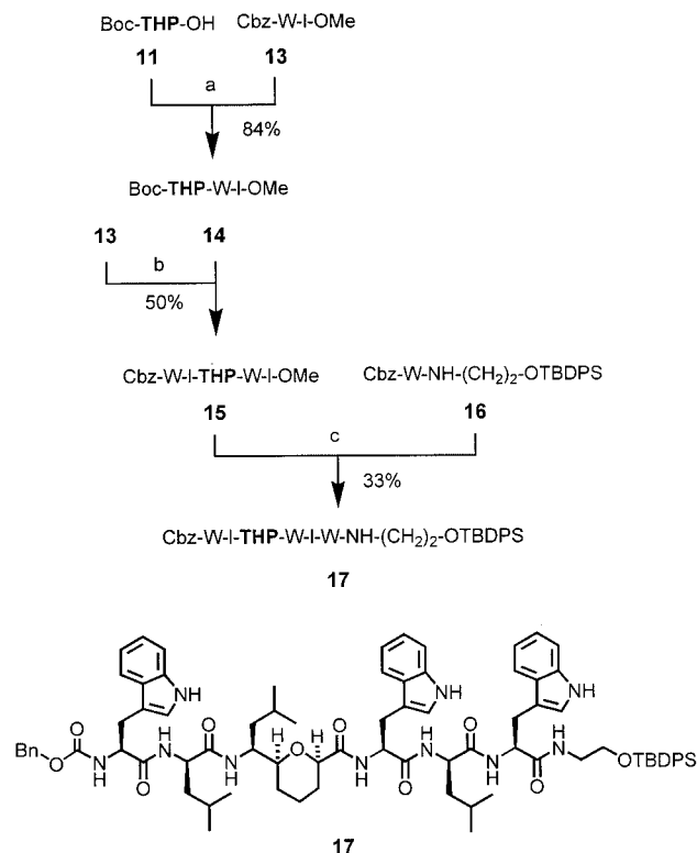
Scheme 4. Synthesis of the hexapeptide 17 by segment coupling in solution. a) i: 13 , H_2 , Pd/C, MeOH, 20 °C; ii: EDC, HOBT, Et_3N , CH_2Cl_2 , 20 °C; b) i: 13 , LiOH, THF/ H_2O , 20 °C; ii: 14 , TFA, CH_2Cl_2 , 20 °C; iii: HOBT, EDC, DIEA, HBtU, CH_2Cl_2 , 20 °C; c) i: 16 , H_2 , Pd/C, MeOH, 20 °C; ii: 15 , LiOH, THF/ H_2O , 20 °C; iii: HOBT, DIEA, HBtU, CH_2Cl_2 , 20 °C.
