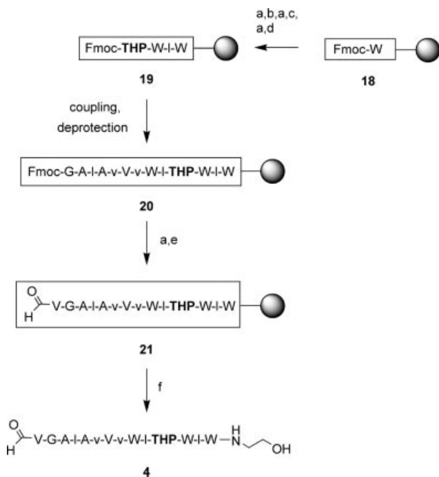
Scheme 5. Solid-phase synthesis of ^{11-12} -THPgA ( 4 ). a) piperidine, DMF, b) Fmoc-I, HOBT, DIEA, HBtU, DMF, c) Fmoc-W, HOBT, DIEA, HBtU, DMF, d) 10 , HOBT, DIEA, HBtU, DMF, e) N -formyl-V, HOBT, DIEA, HBtU, DMF, f) ethanolamine, DMF, 55 °C.
