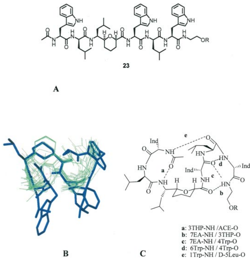
Figure 2. A: Formula structure of compound 23 . B 20 lowest-energy conformations of 23 from NMR calculations. Bold: Structure closest to the average coordinates. C Schematic representation of the multiturn hydrogen-bonding pattern.
