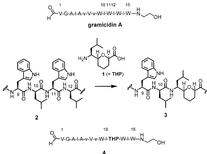
Scheme 1. Generation of the THP-amino-acid gramicidin A hybrid 4 by replacement of positions 11,12 in gA with the THP amino acid 1 ( 2 \rightarrow 3 ).
