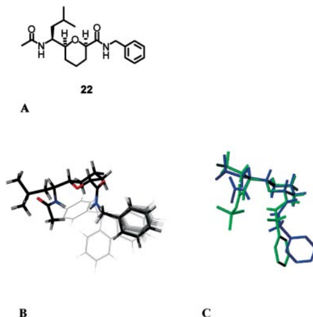
Figure 1. A: Formula structure of 22 . B: Solution structure of 22 : 20 lowest-energy conformations from NMR calculations. Bold: Structure closest to the average coordinates. C: Superposition between solution (blue) and X-ray structure (green).
