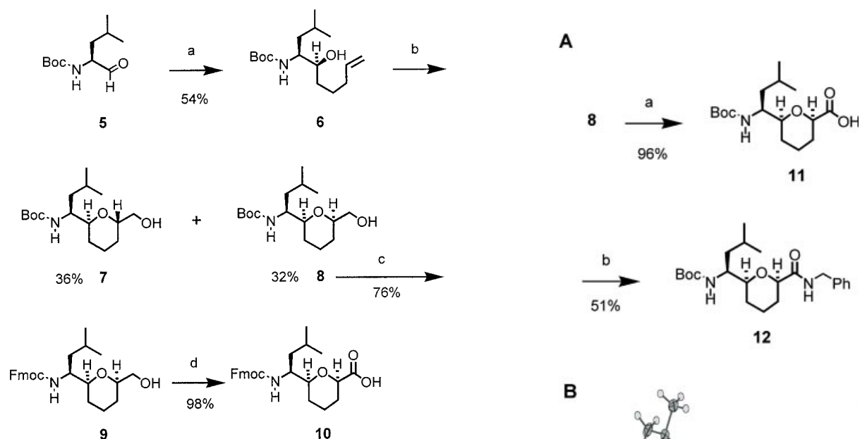
Scheme 2. Synthesis of the N -Fmoc-protected THP amino acid 10 . a) \text{H}_2\text{C}=\text{CH}(\text{CH}_2)_2\text{CH}_2\text{MgBr} , \text{MgBr}_2 , \text{Et}_2\text{O}/\text{CH}_2\text{Cl}_2 , -50\text{ }^\circ\text{C} ; b) i: meta -chloroperbenzoic acid, \text{CH}_2\text{Cl}_2 , 20\text{ }^\circ\text{C} ; ii: camphor sulfonic acid, \text{CH}_2\text{Cl}_2 , 20\text{ }^\circ\text{C} ; c) TFA, \text{CH}_2\text{Cl}_2 , 20\text{ }^\circ\text{C} ; ii: Fmoc-succinimide, \text{NaHCO}_3 , \text{CH}_3\text{CN}/\text{H}_2\text{O} , 20\text{ }^\circ\text{C} ; d) i: (\text{COCl})_2 , DMSO, \text{Et}_3\text{N} , \text{CH}_2\text{Cl}_2 , -60 \rightarrow 0\text{ }^\circ\text{C} ; ii: \text{NaClO}_2 , \text{NaH}_2\text{PO}_4 , amylene, t\text{BuOH}/\text{H}_2\text{O} , 20\text{ }^\circ\text{C} .
